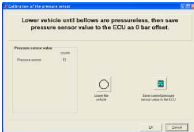
Abb. Menu "Calibrate the pressure sensor" in the Diagnostic Software
